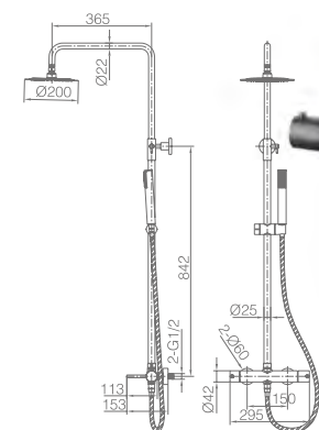
Black gun metal stainless steel S.304 telescopic bar. Black gun metal stainless steel S.304 round shower head Ø20 cm, extra flat design and antilime system. Elevated adjustable support handle. Round 1 position handle shower. Black gun metal brass single-lever with integrated flow-diverter. Medium flow rate 12 l/min. PVC hose 150 cm. Ceramic cartridge Ø35 mm.
