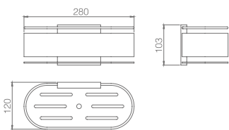
Ref.: ADN008/NG Anga front soap holder. Matt back finish. S.304 Steel.
