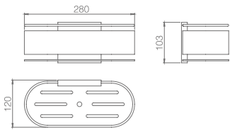
Ref.: ADN008/NOR Anga front soap holder. Matt back - rose gold finish. S.304 Steel.
