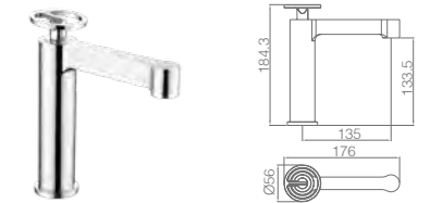
Single-lever basin. Brass body. Chrome finish. Ceramic cartridge Ø26 mm TOP. Flexible hoses 3/8".
