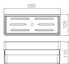
Ref.: ABL006 Material: PVC. Finished: Matt white.
