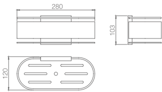
Ref.: ADN008/NQ Anga front soap holder. Brushed nickel finish. S.304 Steel.
