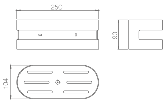
Ref.: ADL012/BL Iman front soap holder. Matt white finish. S.304 Steel.
