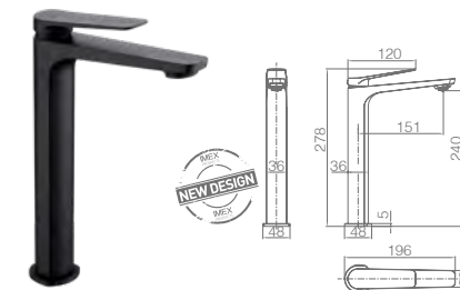
Single-lever high basin. Brass body. Matt black finish. Ceramic cartridge Ø26 mm TOP. Flexible hoses 3/8".
