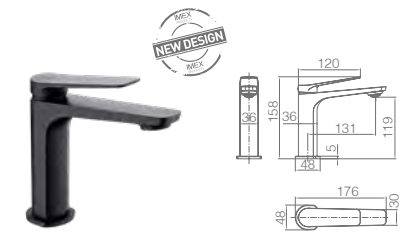
Single-lever basin. Brass body. Matt black finish. Ceramic cartridge Ø26 mm TOP. Flexible hoses 3/8".
