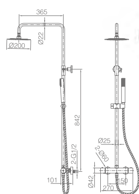
Black gun metal stainless steel S.304 telescopic bar. Black gun metal stainless steel S.304 round shower head Ø20 cm, extra flat design and antilime system. Elevated adjustable support handle. Round 1 position handle shower. Black gun metal brass thermostatic with integrated flow-diverter. Medium flow rate 12 l/min. PVC hose 150 cm. Thermostatic cartridge TURN CLEAN SYSTEM.
