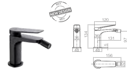
Single-lever bidet. Brass body. Matt black finish. Ceramic cartridge Ø26 mm TOP. Flexible hoses 3/8".
