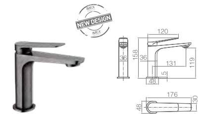
Single-lever basin. Brass body. Black gun metal finish. Ceramic cartridge Ø26 mm TOP. Flexible hoses 3/8".
