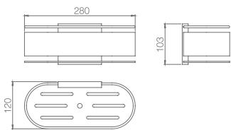
Ref.: ADN008/BL Anga front soap holder. Matt white finish. S.304 Steel.
