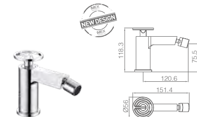
Single-lever bidet. Brass body. Chrome finish. Ceramic cartridge Ø26 mm TOP. Flexible hoses 3/8".
