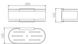
Ref.: ADN008 Anga front soap holder. Chrome finish. S.304 Steel.
