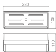
Ref.: ANG005 Material: PVC. Finished: Matt black.
