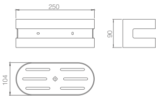
Ref.: ADL012/NQ Iman front soap holder. Brushed nickel finish. S.304 Steel.
