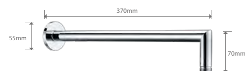
Ref.: BPF002 Round wall tube (90°). Chrome brass.
