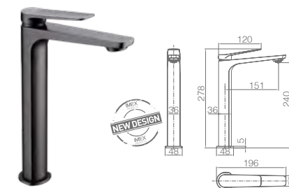
Single-lever high basin. Brass body. Black gun metal finish. Ceramic cartridge Ø26 mm TOP. Flexible hoses 3/8".
