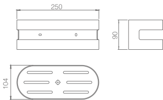
Ref.: ADL012 Iman front soap holder. Chrome finish. S.304 Steel.
