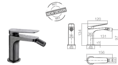
Single-lever bidet. Brass body. Black gun metal finish. Ceramic cartridge Ø26 mm TOP. Flexible hoses 3/8".
