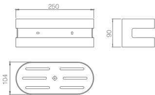
Ref.: ADL012/NG Iman front soap holder. Matt black finish. S.304 Steel.
